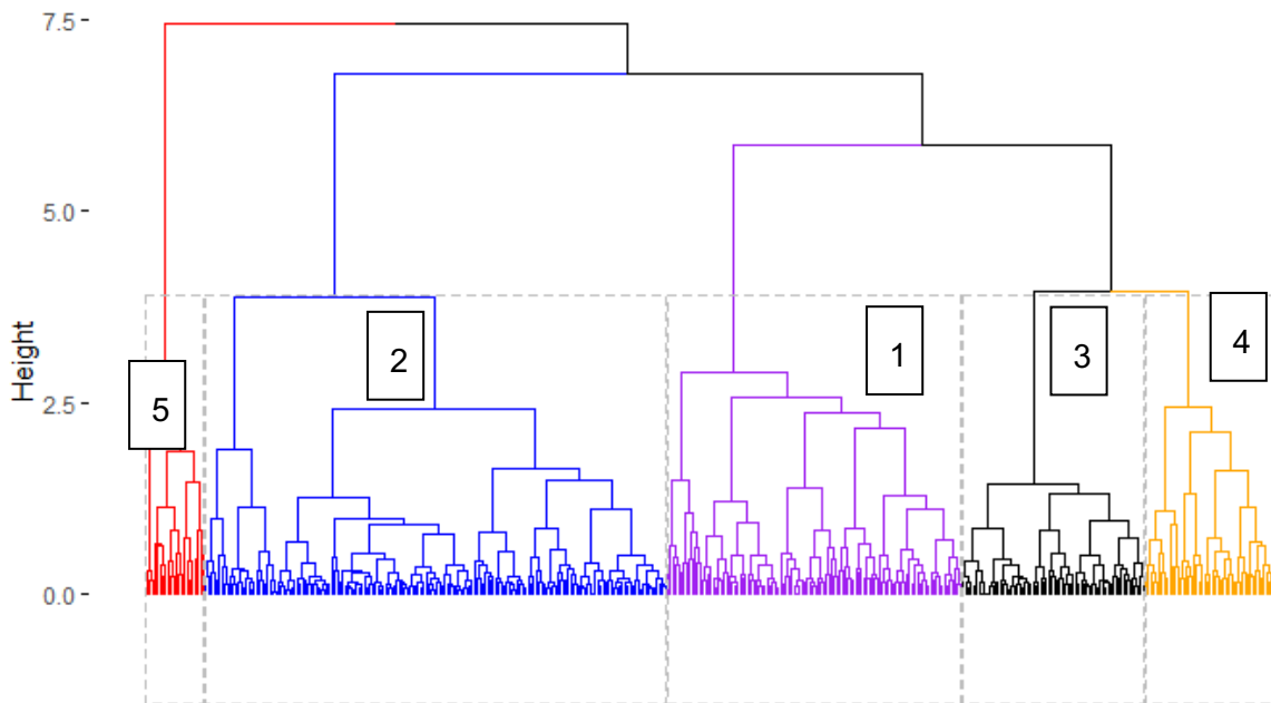
Cluster Dendrogram
