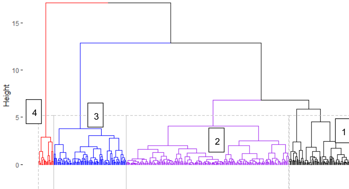
Cluster Dendrogram
