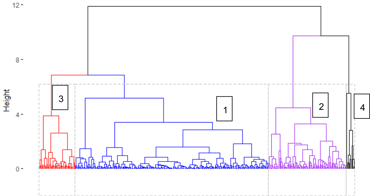
Cluster Dendrogram
